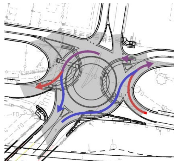
Conceptual roundabout design for the intersection of Idaho Street and 13th Avenue
